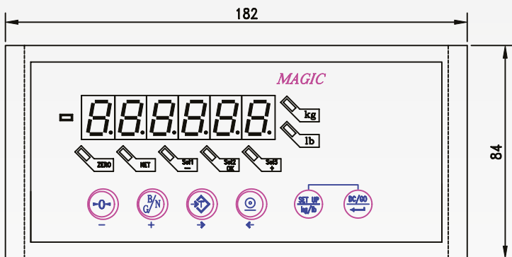
Front Panel RP15-M ABS Unit
