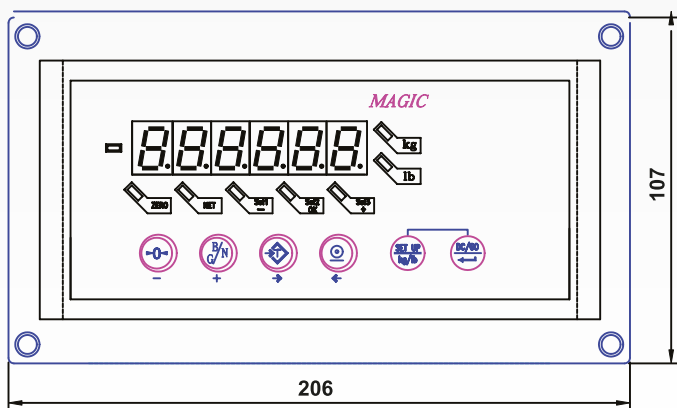
Front Panel RP15-M SS Unit
